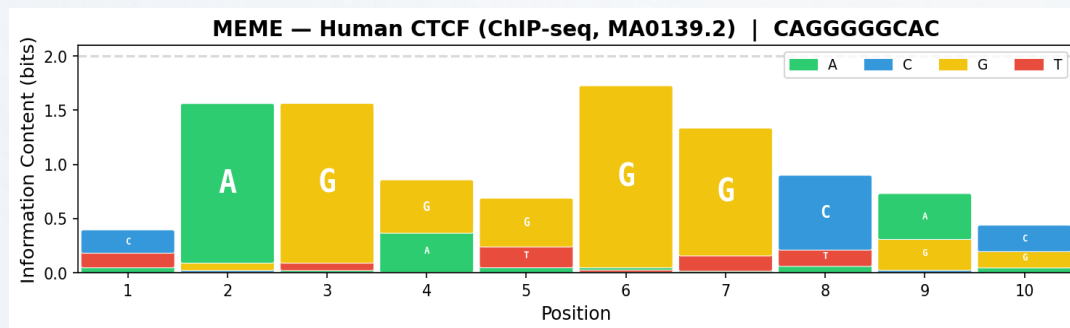
MEME Sequence Logo — Human CTCF (ChIP-seq, MA0139.2)
